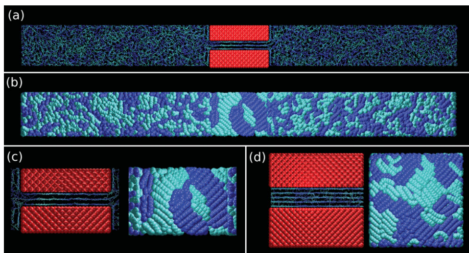
Figure 2. A comparison of GCMC and NPT ensemble simulations.
