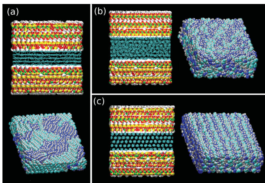
Figure 3. The evidence from atomistic simulation.
