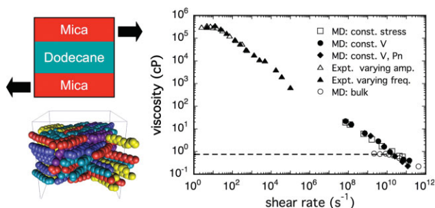
Figure 1. Molecular dynamics simulations of nanoconfined dodecane by Cui et al. 15,32
